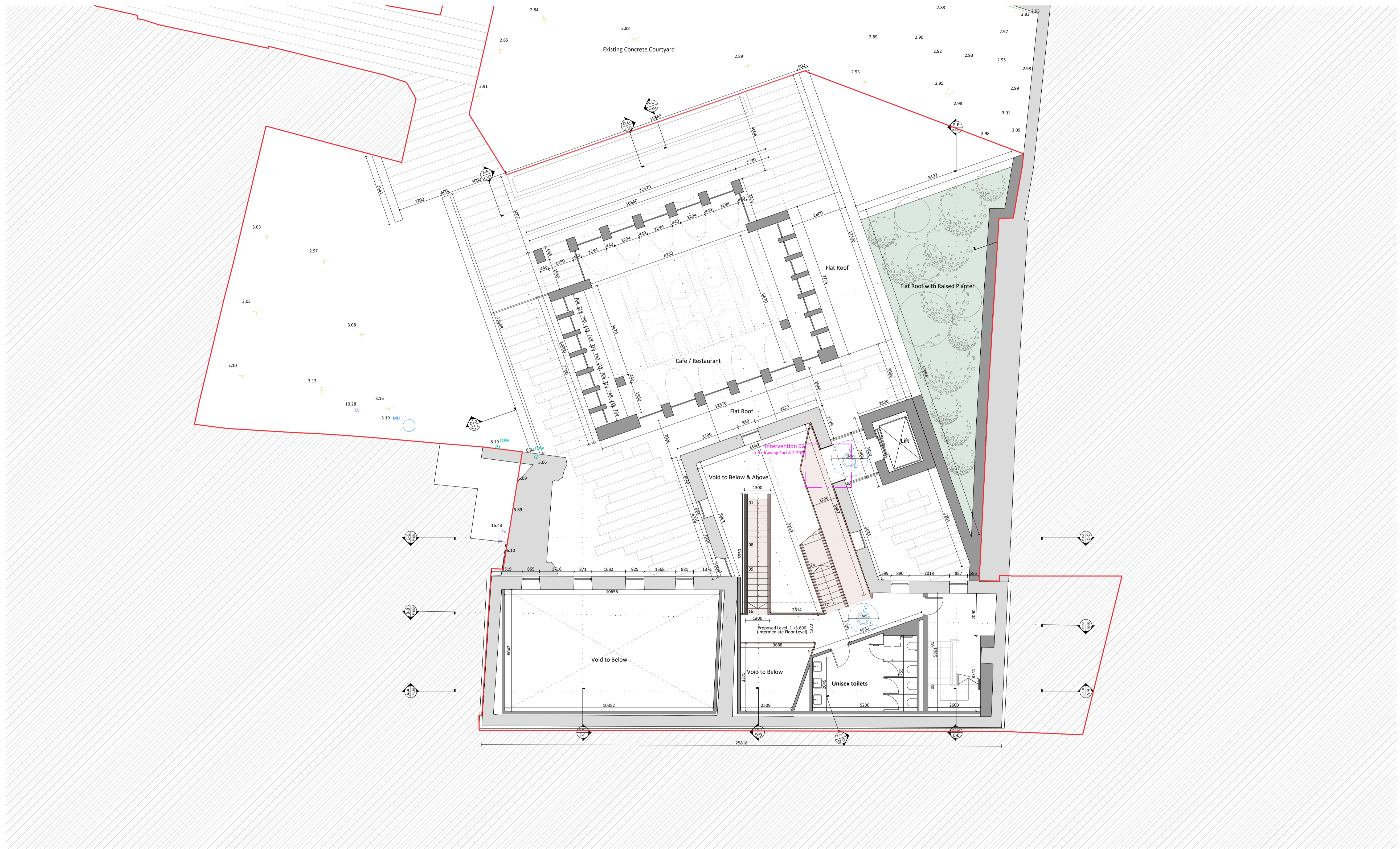
01 Level -1 (Basement) Floor Plan As Proposed Scale: 1:100
